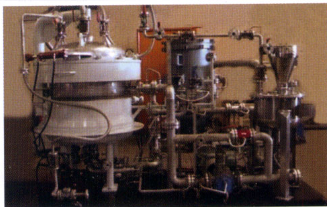
Skid mounted unit with piping and valves
