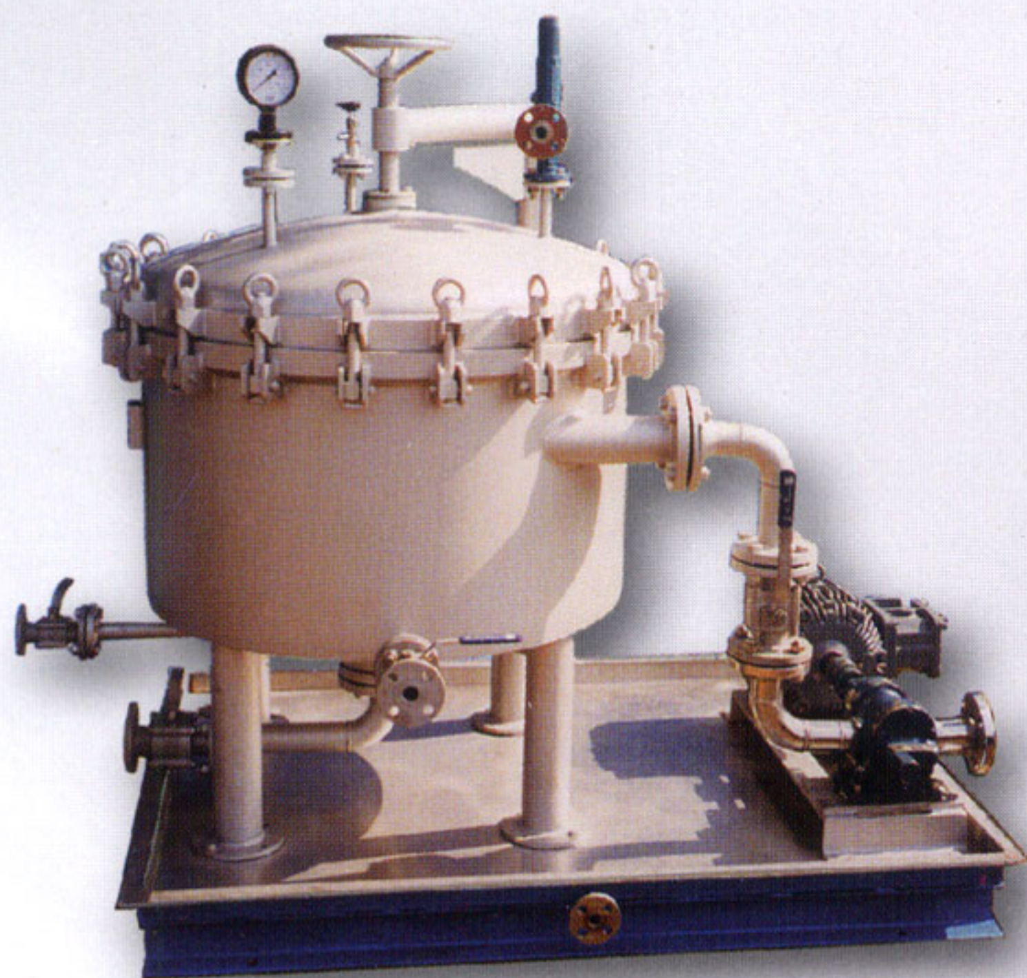
Standard Model Horizontal Plate Closed Filter
